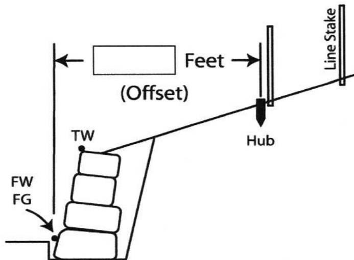
Uphill Staking (Stakes above wall)
