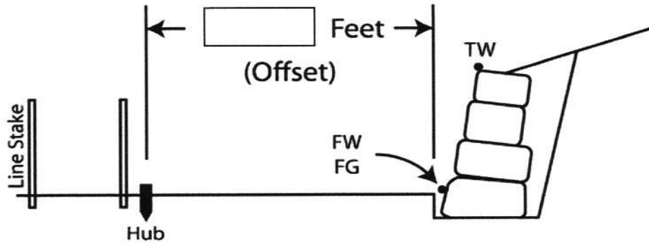
Downhill Staking (Stakes below wall)
